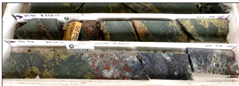
Figure 1. Cut diamond core from YQ-25-007 at the Yoquivo Project highlighting a very high grade silver-bearing sulphide vein (black/grey) with accessory hematite (brown) and quartz (white). Assays for this interval graded 0.59 metres at 2,584g/t AgEq 1 - 1,935g/t Ag & 8.5g/t Au from 312.38m.
