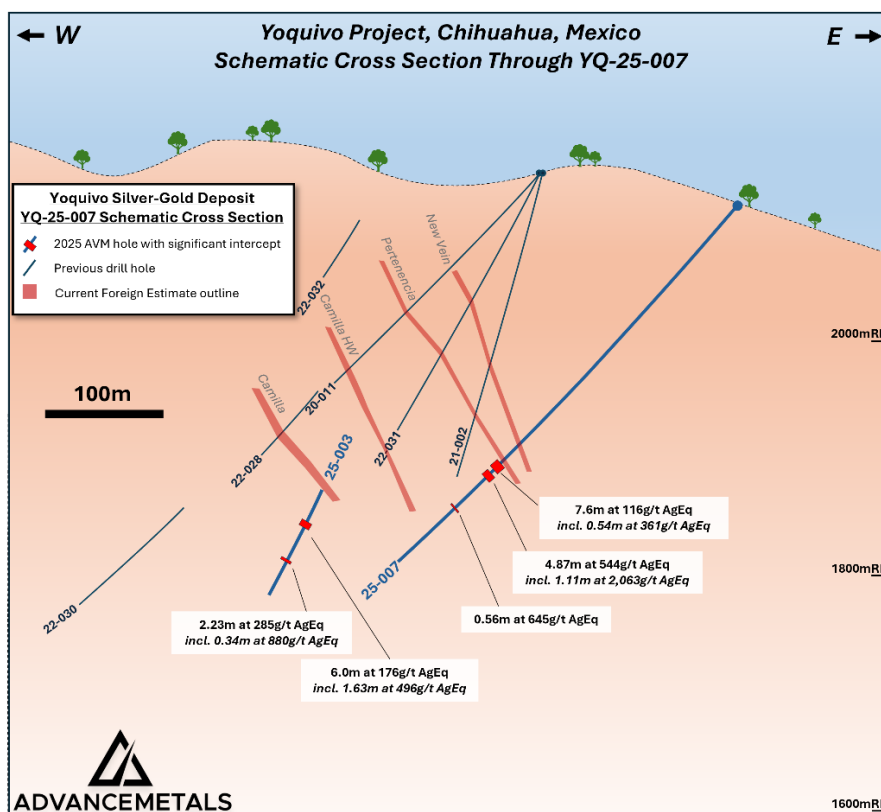
Figure 2. Schematic cross section ( \pm 20\text{m} , looking north) showing previous drilling 2 and the approximate outline of the existing Foreign Estimate 2 , along with significant down hole intersections for YQ-25-007 (see Table 1 & 2 for full details) and the bottom portion of YQ-25-003 (previously reported 4 ).
