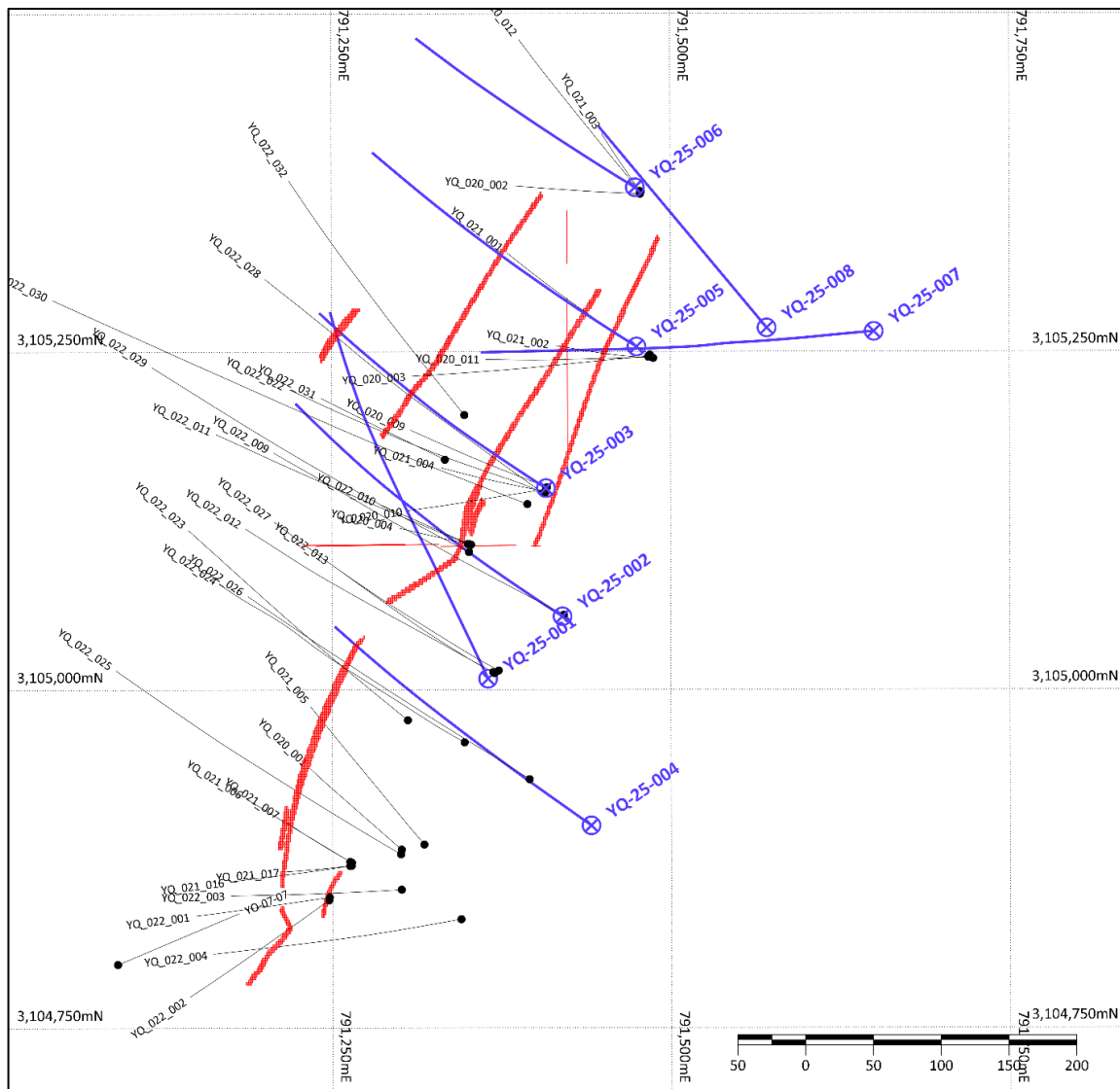
Figure 4. Plan of the Pertenenencia area showing previous drilling 2 and recently completed diamond holes (blue). A level section of the current Foreign Estimate 2 for Yoquivo at 1,960mRL is also shown in red. Full details for the recent drilling are given in Table 1 .
