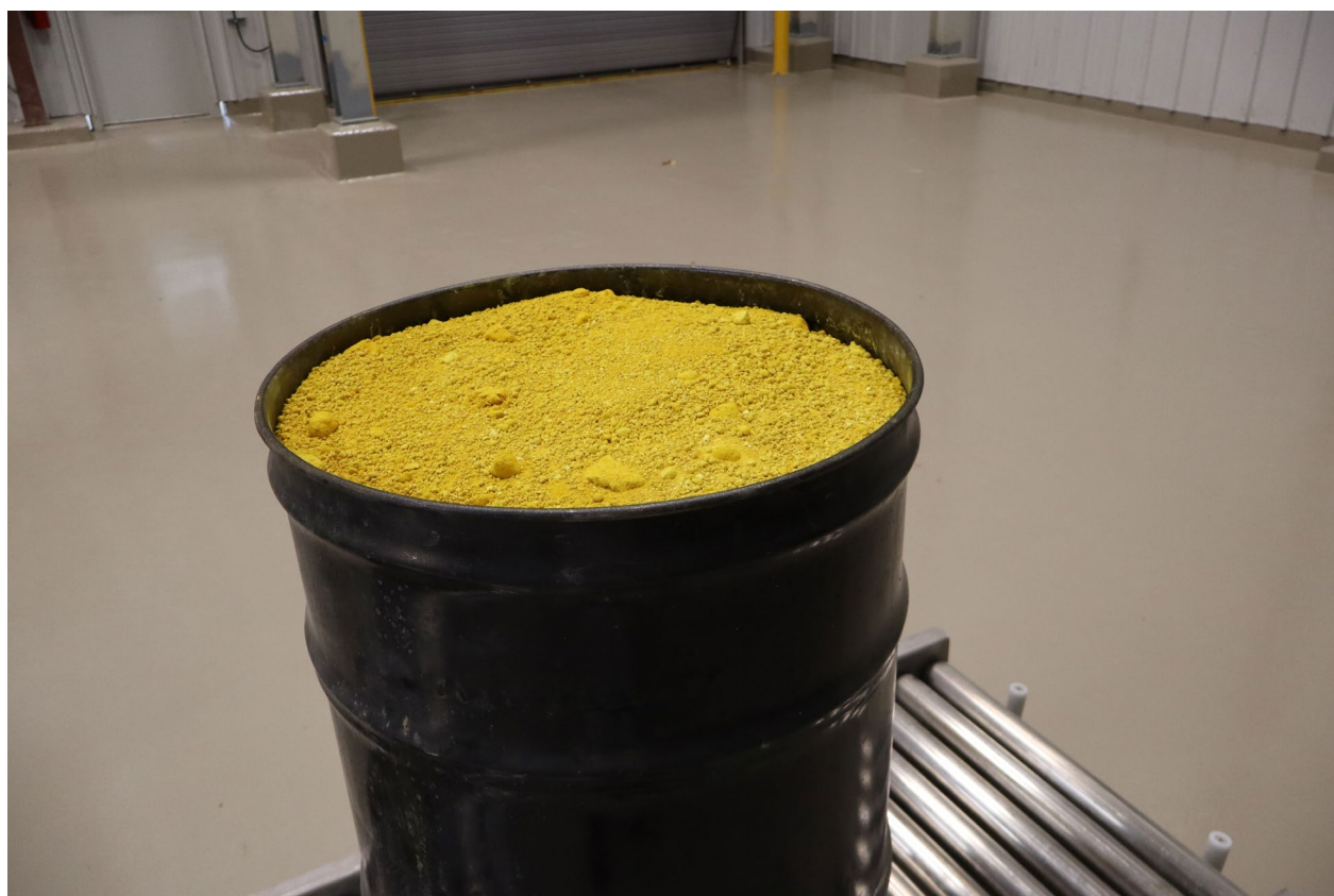
First Drum of Dried Yellowcake – Lance Project
