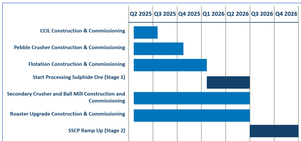
Figure 3: SSCP Timeline
