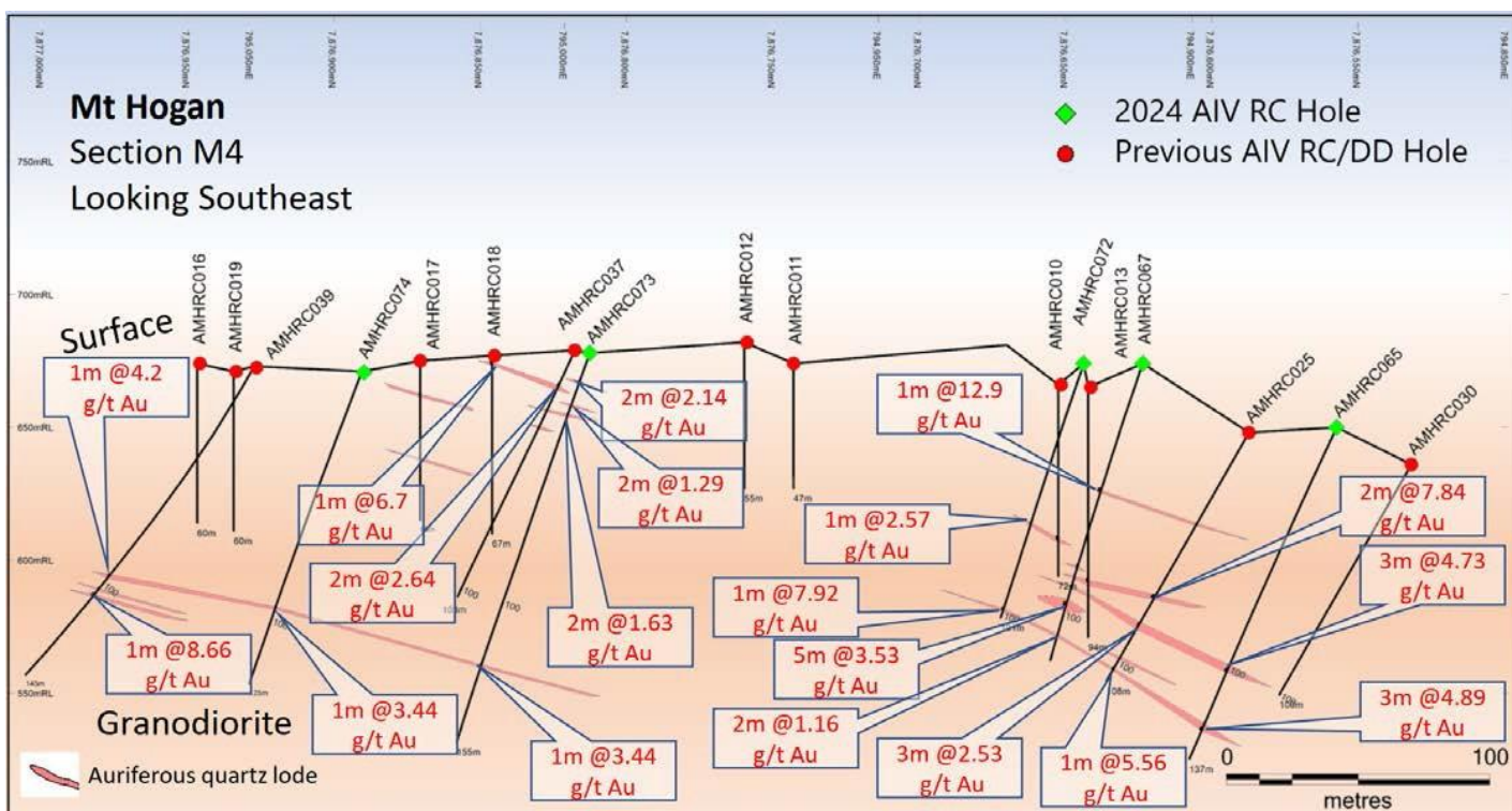
Figure 6. Mt Hogan Historic Gold Mine Cross Section M4
