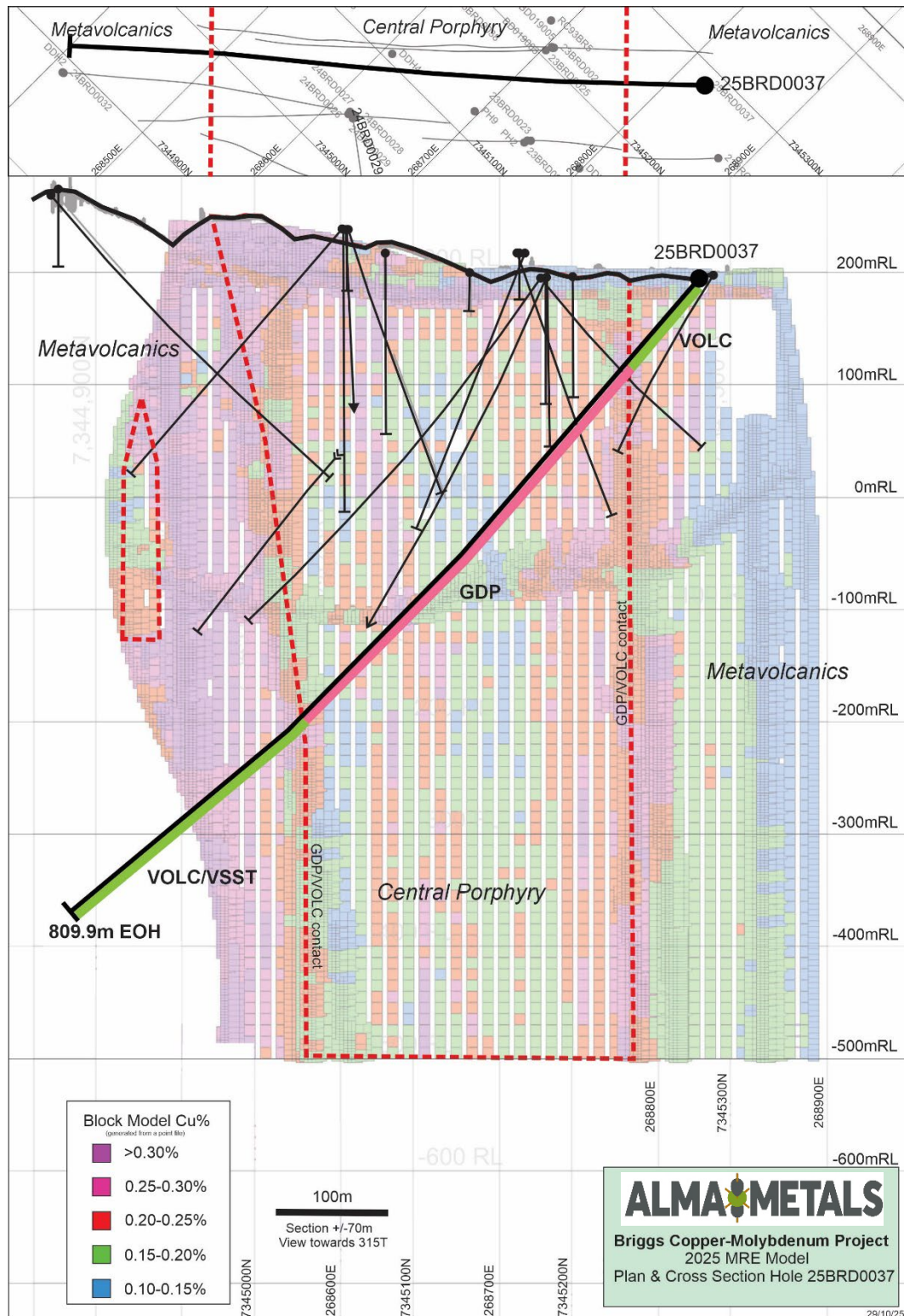
Figure 2. Cross Section showing down-hole geology in 25BRD0037 and the estimated copper grades from the MRE block model.
