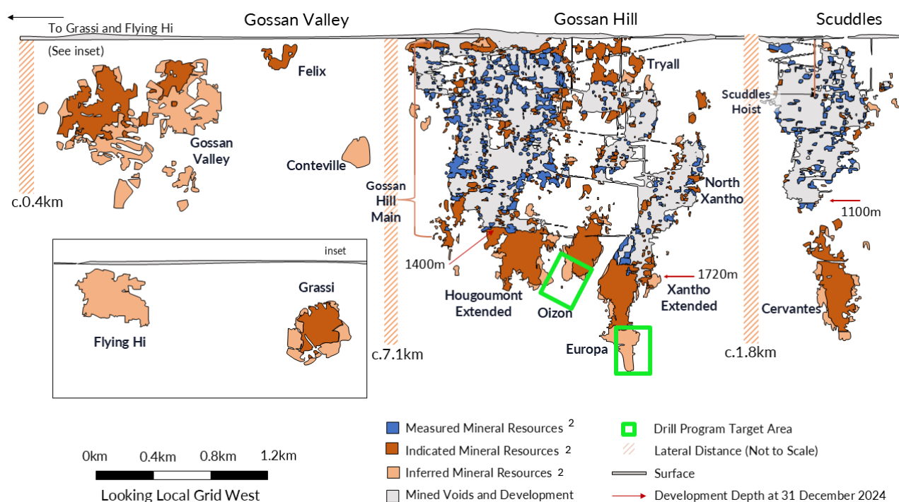
Figure 1: Golden Grove long-section highlighting Ozion and Europa drilling target areas.
