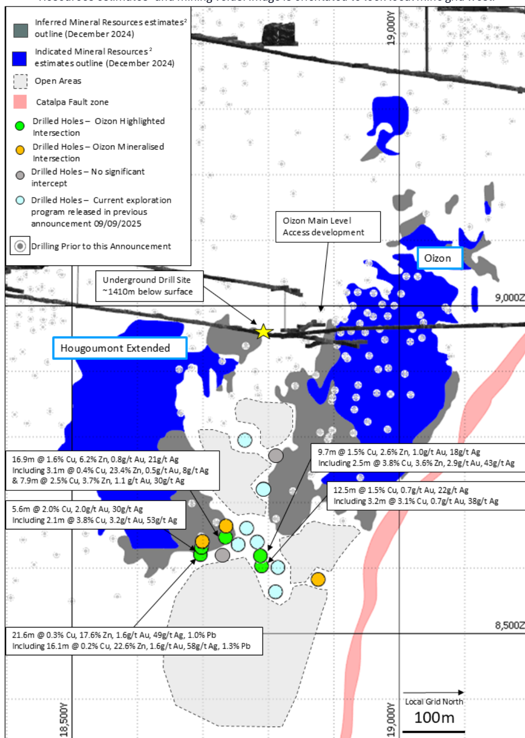
Figure 3: Long-section of Oizon and Hougoumont Extended – showing pierce points of highlighted assays results from holes reported in this release as well as the pierce point locations of historic drilling in relation to existing Mineral Resources estimates 2 and mining voids. Image is orientated to look local mine grid west.
