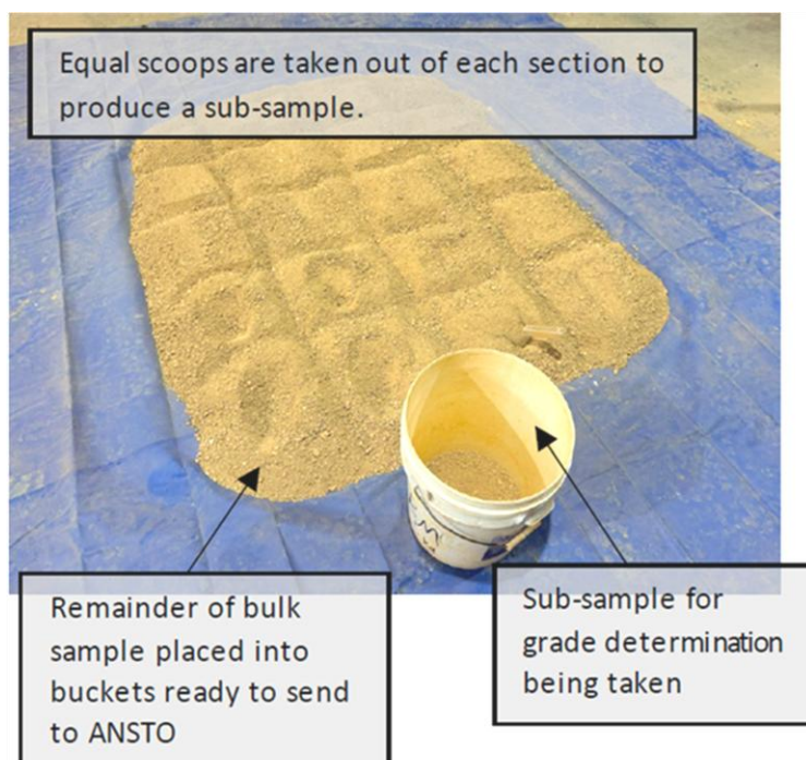
Figure 3 (above): Increment subsampling of the 100kg ANSTO sample crush and ground to less than 5mm.
