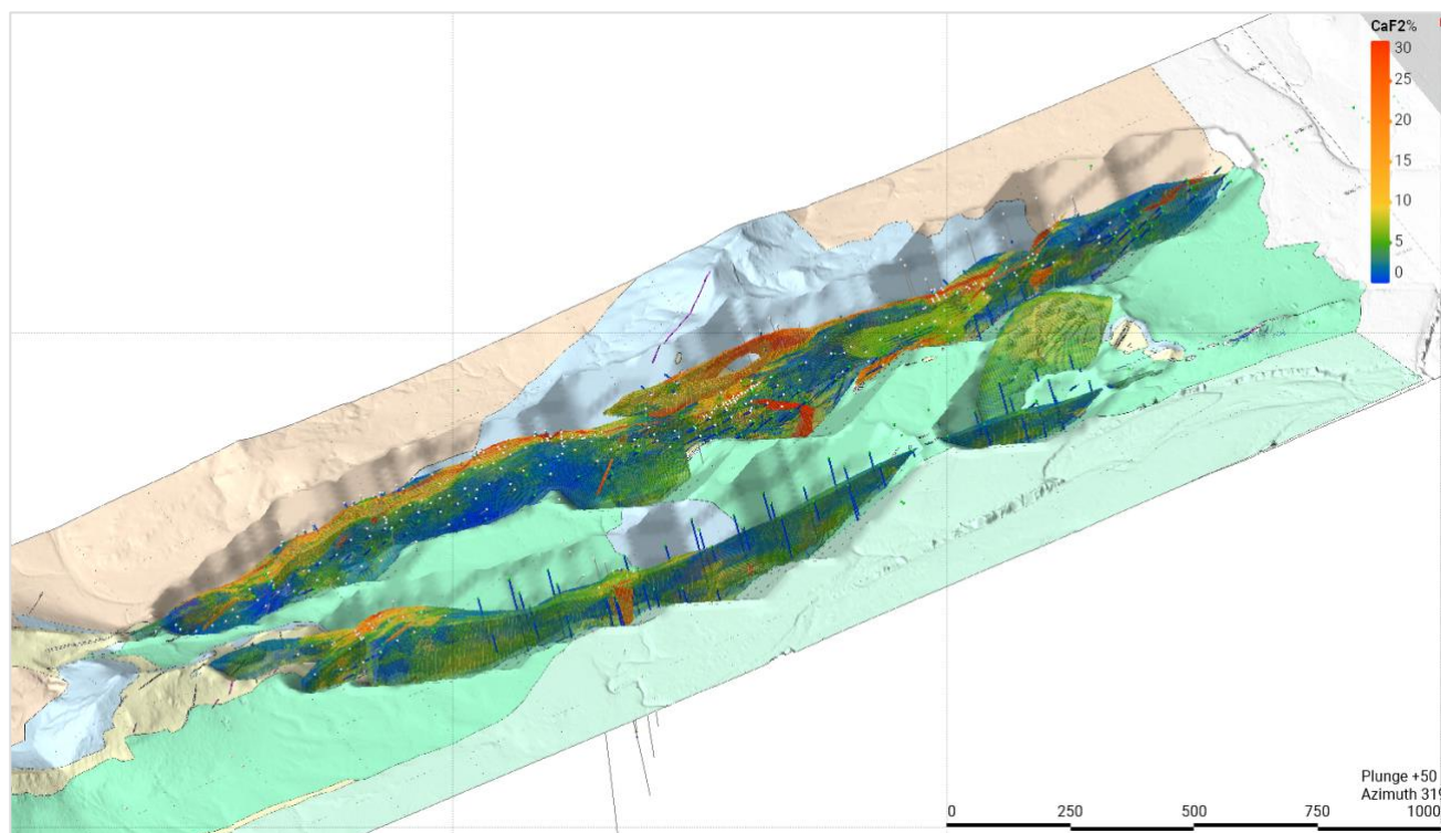
Figure 14: Block model and drilling within the constraining pit shell (source: SRK)
