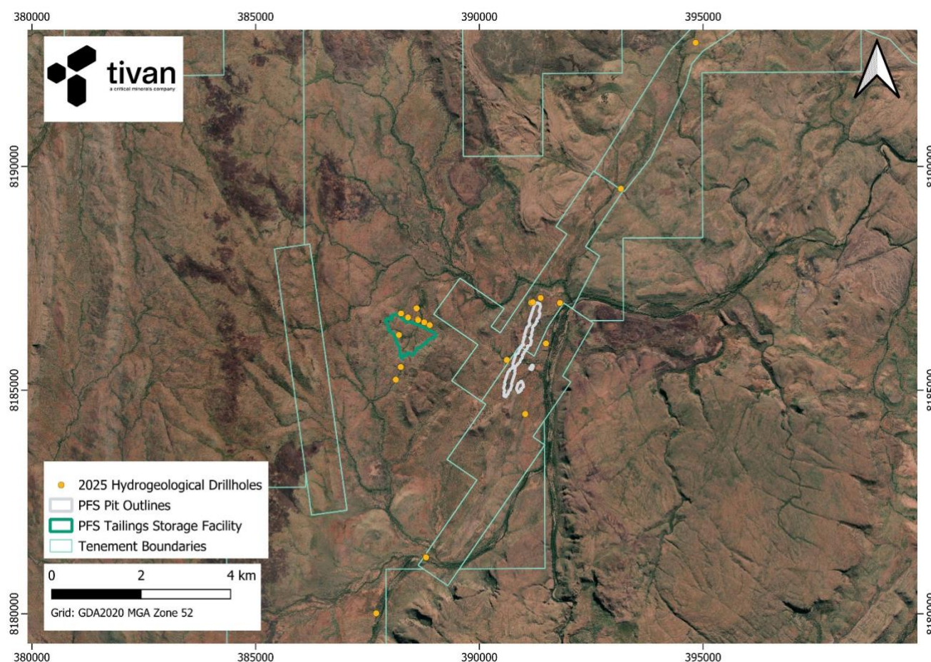
Figure 12: Location of hydrogeological drilling completed in 2025
