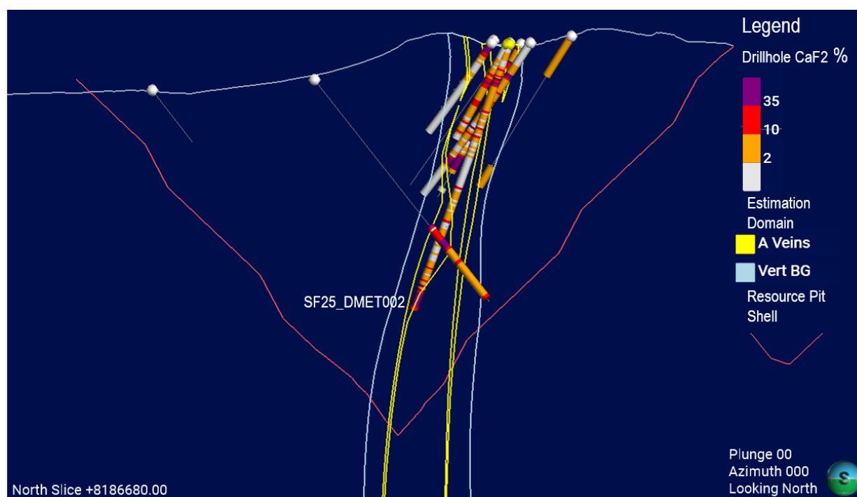
Figure 5: Cross section of metallurgical drilling from Speewah geological model.
