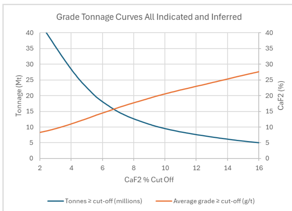
Figure 20: Grade and tonnage curves – all Mineral Resource material (source: SRK)
