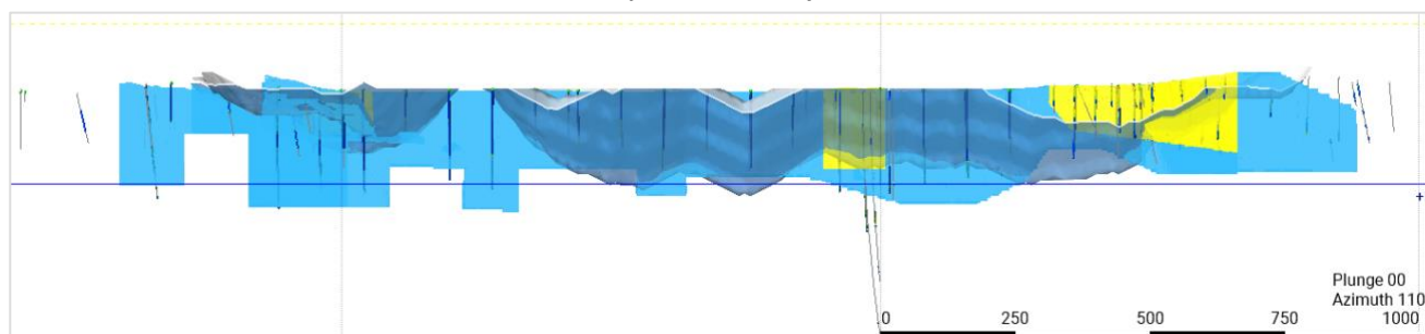
Figure 19: Classification, Resource reporting pit shell and drilling – long section looking east, G Vein (source: SRK)
