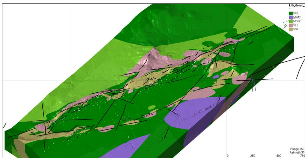
Figure 17: SRK-interpreted deposit-scale fault architecture and lithology at surface (source: SRK)
