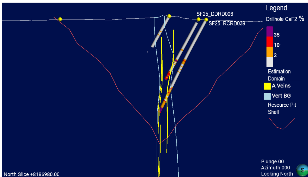
Figure 11: Cross section of A-Vein North extension drilling from Speewah geological model
