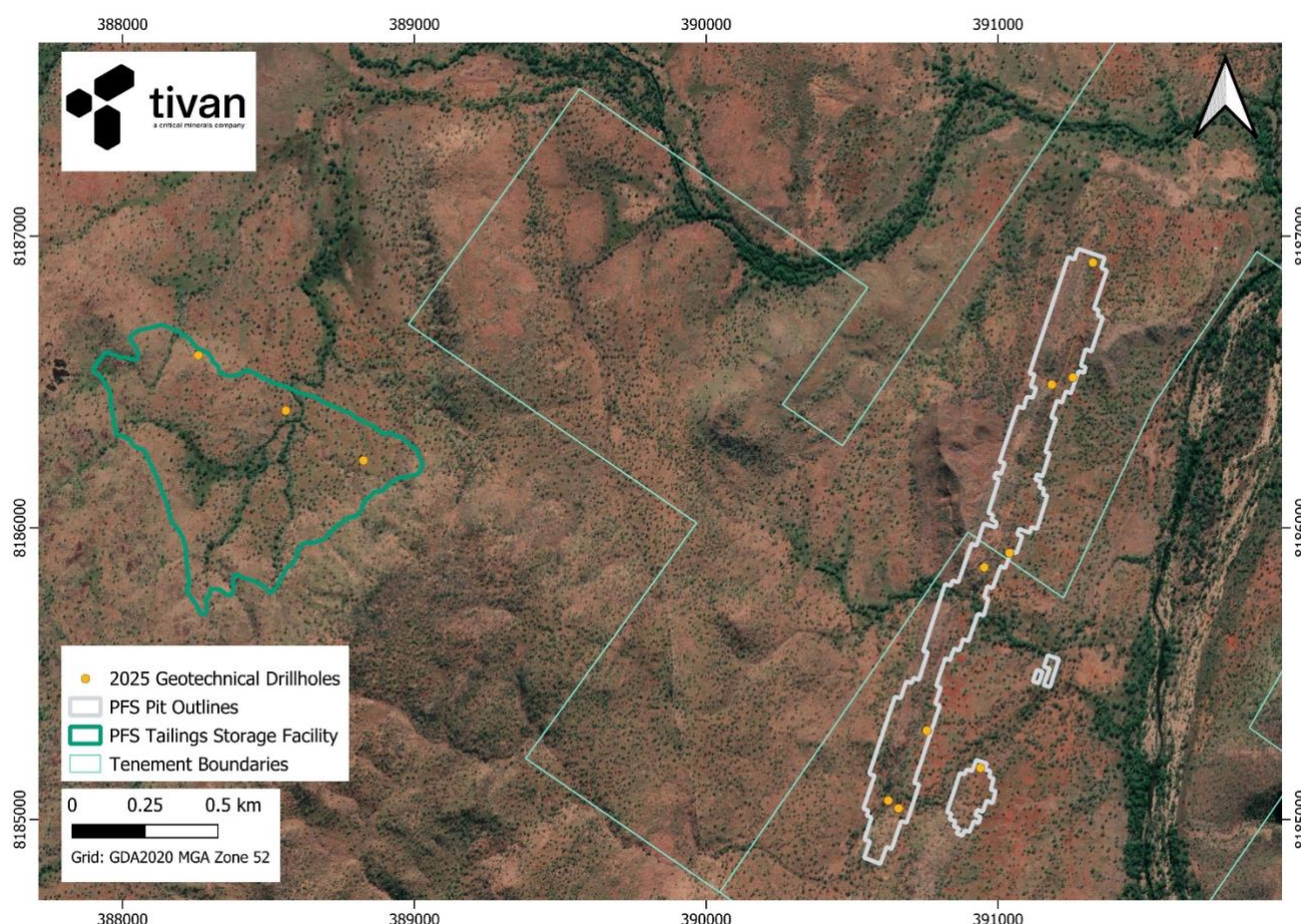
Figure 13: Location of geotechnical drilling completed in 2025
