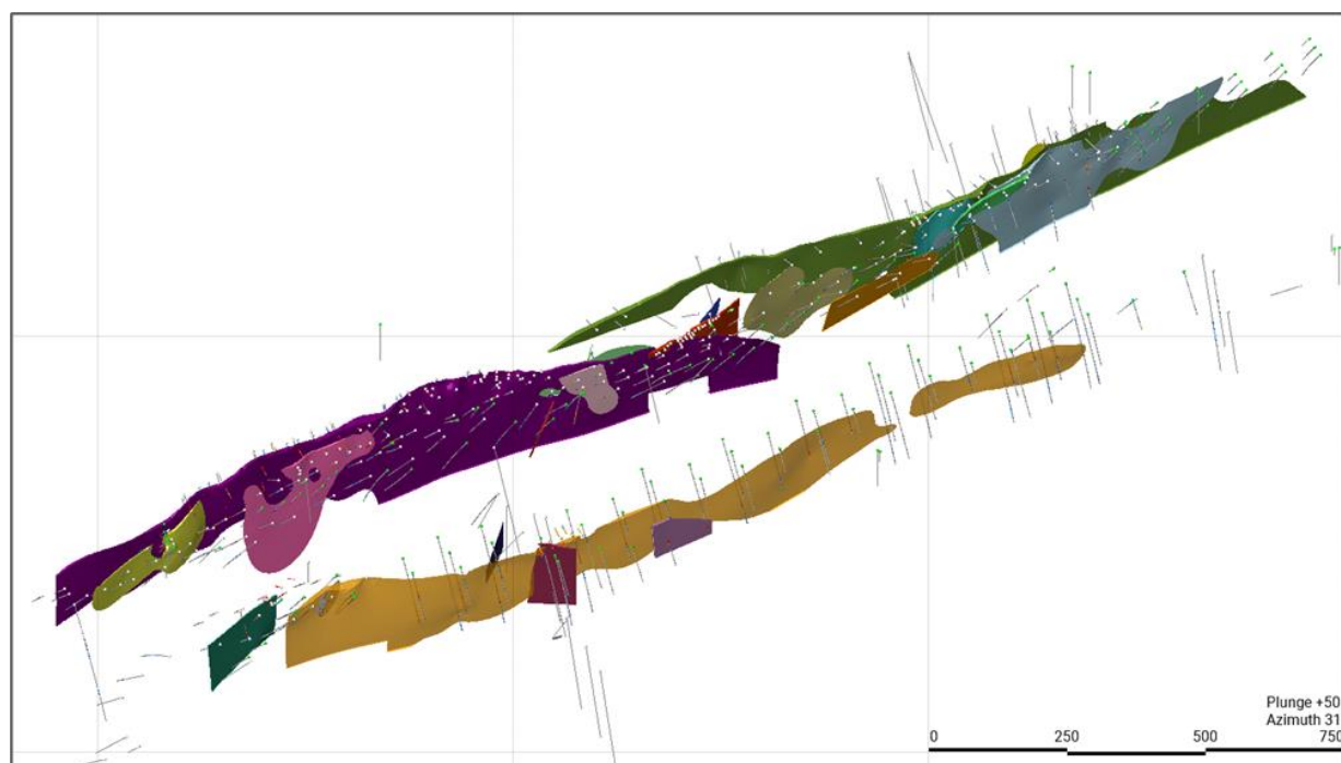
Figure 15: Modelled veins and drilling – perspective view looking north-northwest (source: SRK)
