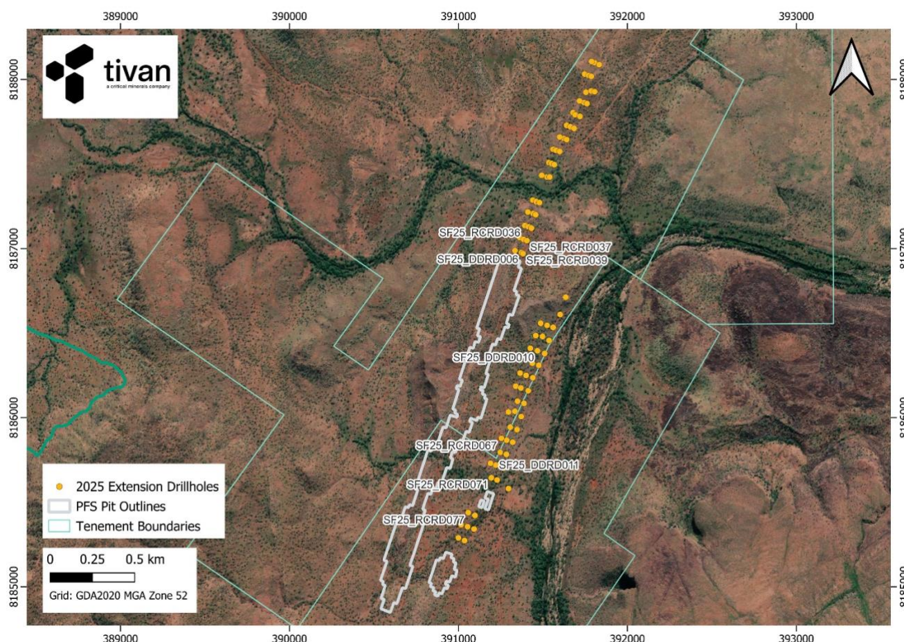
Figure 7: Location of extension drilling completed in 2025 (drill holes with significant intercepts are labelled)
