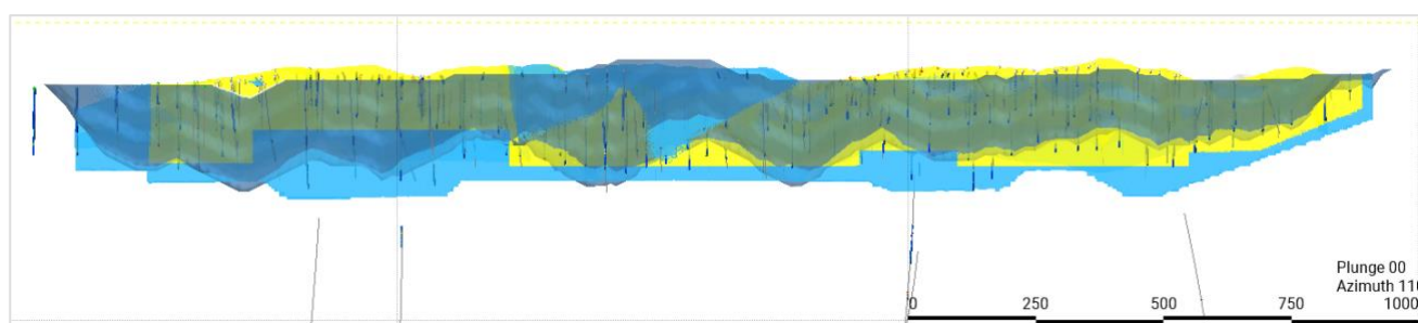
Figure 18: Classification, Resource reporting pit shell and drilling – long section looking east, A and B Veins (source: SRK)
