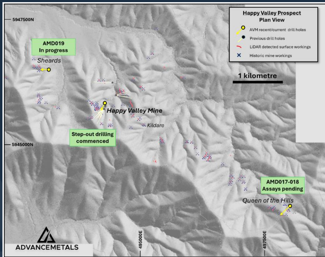
Figure: Plan of the southeastern portion of the Myrtleford Project highlighting current status of drilling in the Happy Valley Trend (ASX AVM 21 January 2026).
