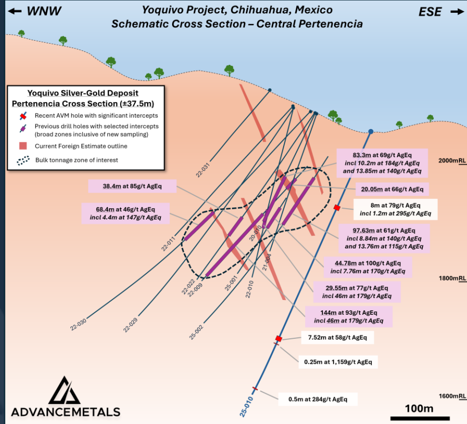
Figure: Schematic cross section looking NNE showing significant down hole intersections for recent AVM hole YQ-25-010 and selected broad intervals emerging from recent historic core resampling (ASX AVM 6 February 2025)
