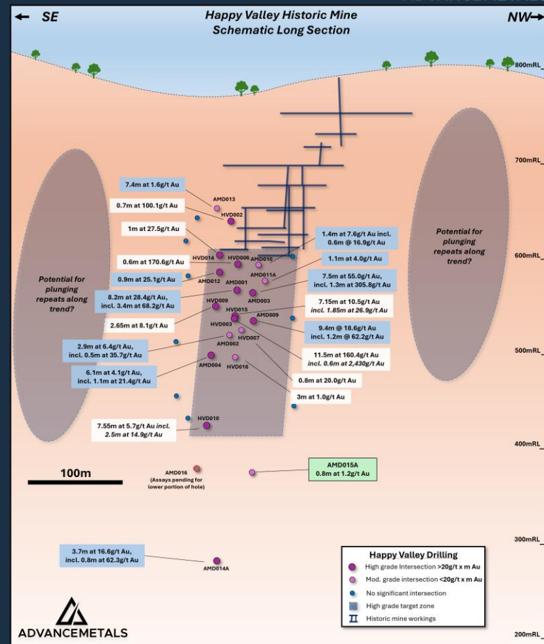
Figure: Schematic long section looking southwest (ASX AVM 21 January 2026) showing previously drilling by Serra Energy Metals at Happy Valley ("HVD" holes) along with recent drilling by AVM ("AMD" holes)
