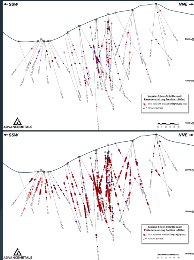
Figure: Schematic long sections of the Pertenencia area at Yoquivo showing drilling with down hole assays of 200g/t AgEq (top) and 20g/t AgEq (bottom) (ASX AVM 6 February 2025).
