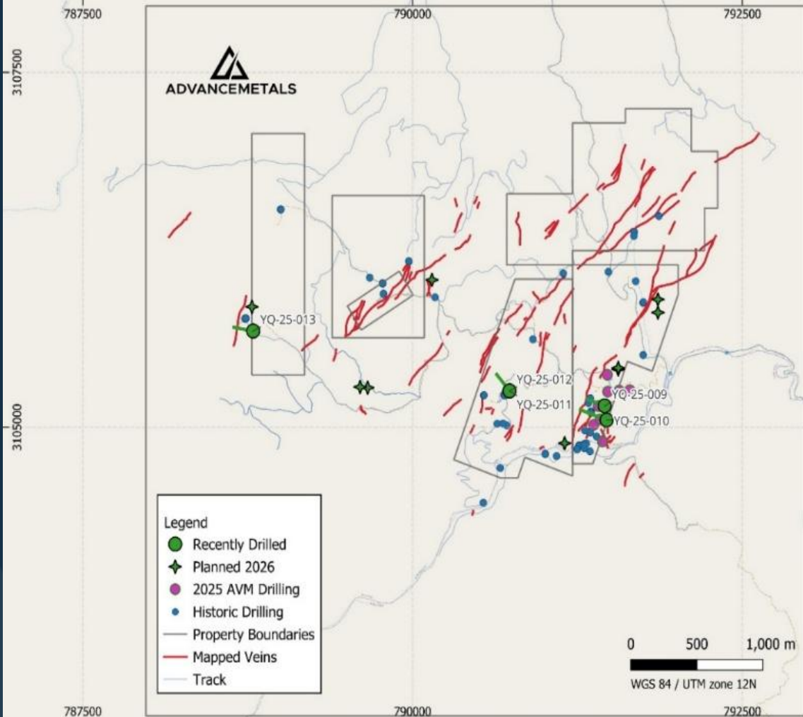
Figure: Plan of the Yoquivo Silver-Gold Project showing mapped veining and the location of hole recent and planned drilling locations (ASX AVM 22 January 2026).
