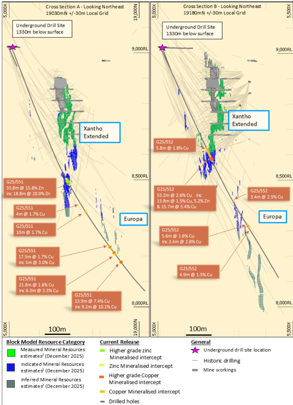
Figure 7: Cross-section view looking local grid northeast displaying Europa and Xantho Extended, sulphide lenses, and mining voids. Highlighted drill hole traces reported in this release and historic drilling.
